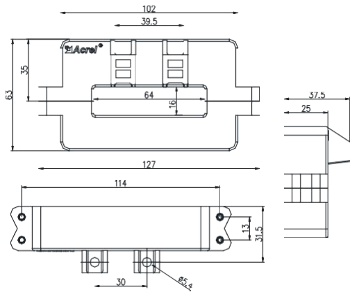
AHKC-K (200A/5V) aperture Φ64*16mm
