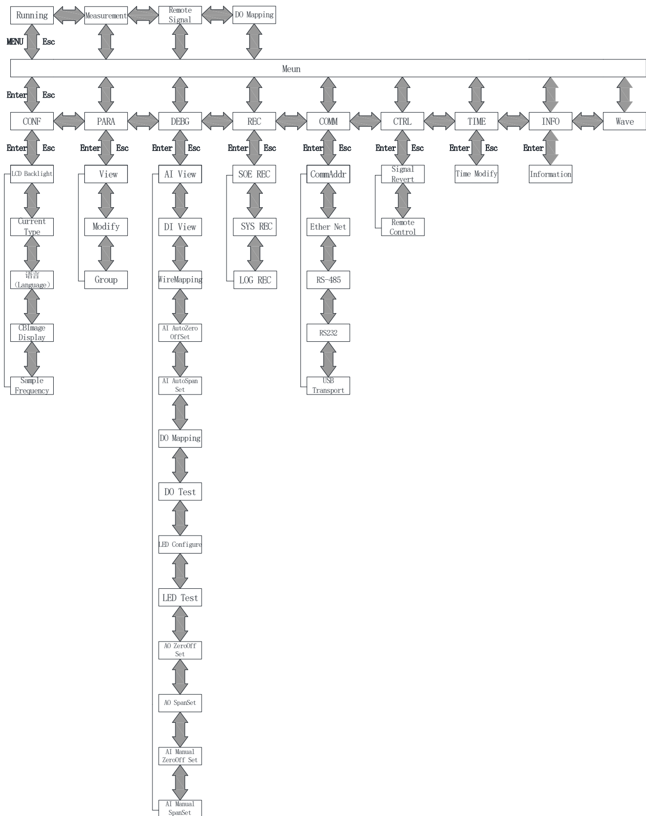
Figure 3.7 Navigation diagram
