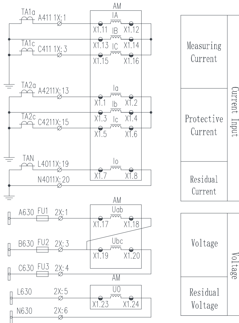
Figure 5.3 2PT & 2CT Wiring
