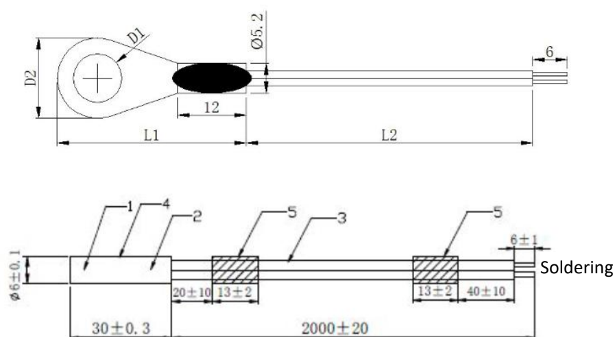
4) Temperature sensor (unit: mm)
