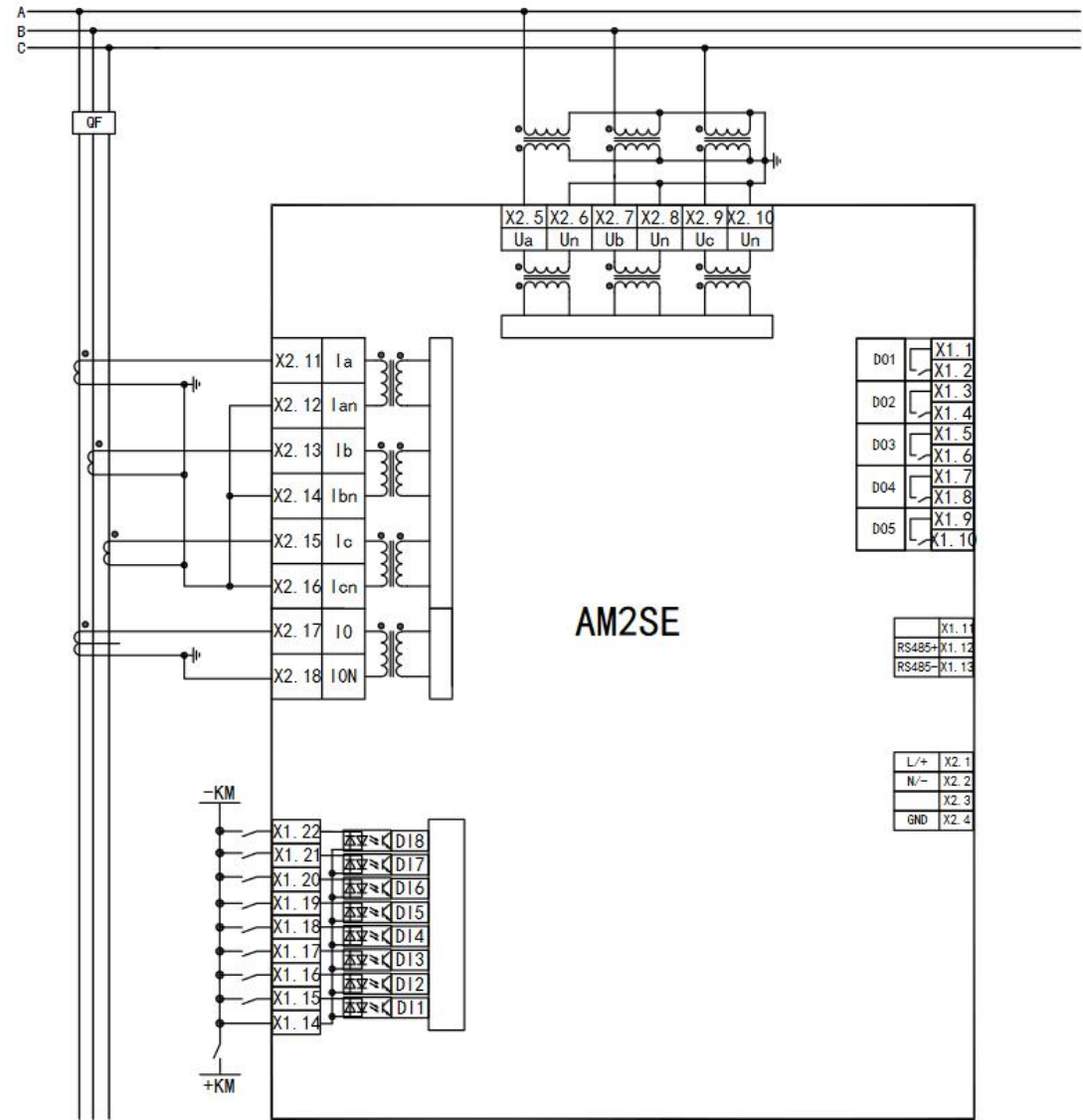
Fig. 5.2 Typical application diagram
