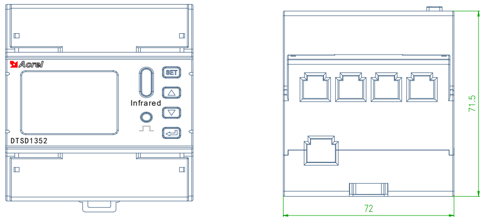
Figure 2 DTSD1352 - 4S dimension
