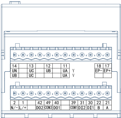
Figure 4 DTSD1352-4S (2DI2DO) module reverse wiring terminals
