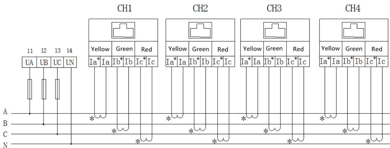
Figure 7 Three-phase four-wire voltage and current are directly connected
