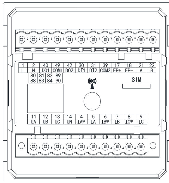
Figure 10 APM510 extended 4G/NB wiring diagram
