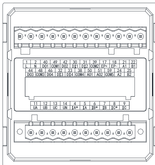
Figure 8 APM510 extended K/2M/2C wiring diagram
