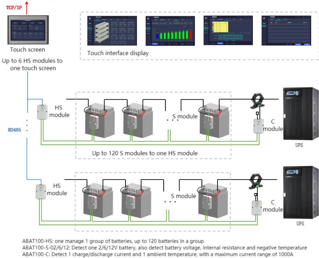
Fig.2 Network plan 1
