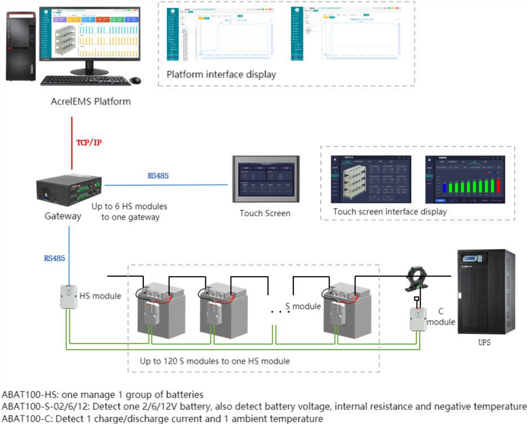
Fig.3 Network plan 2
