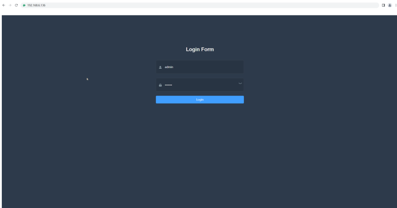
Figure 4 Login Interface
