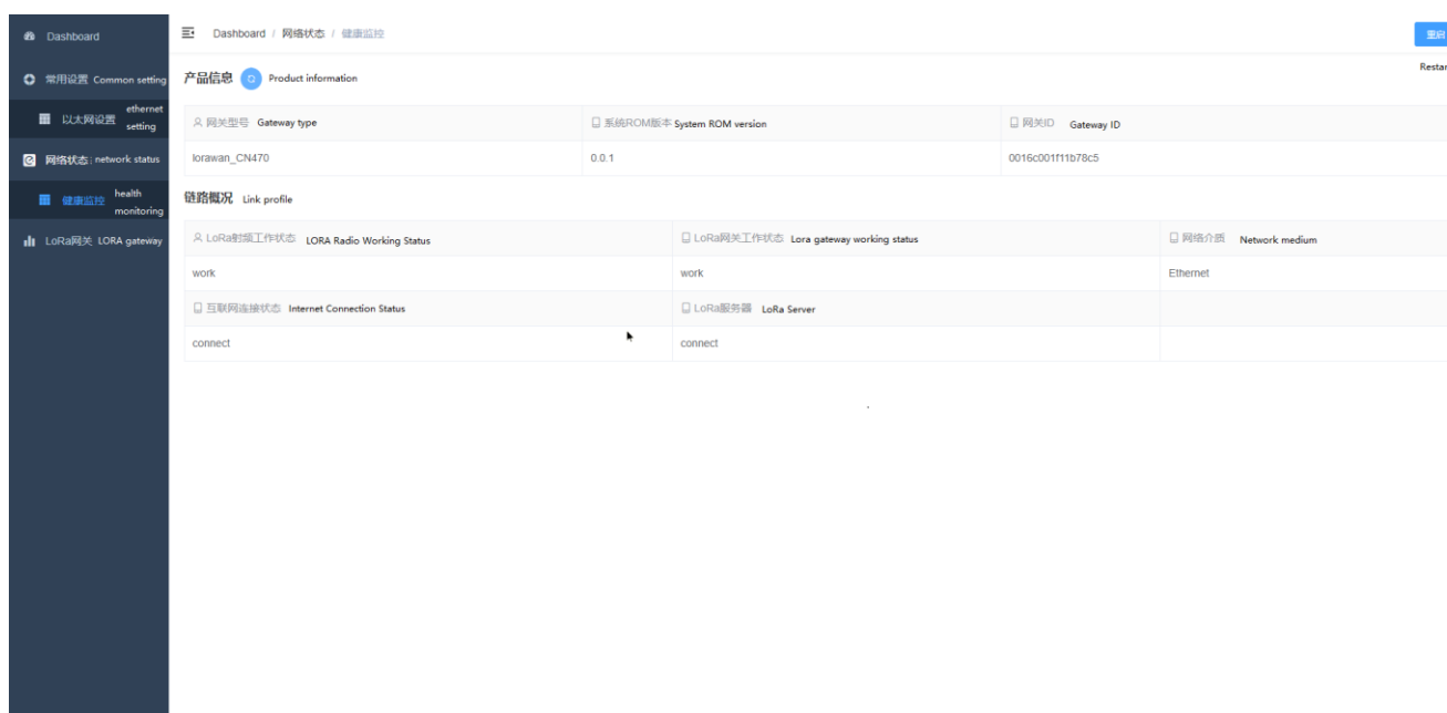
Figure 7 Health Monitoring
