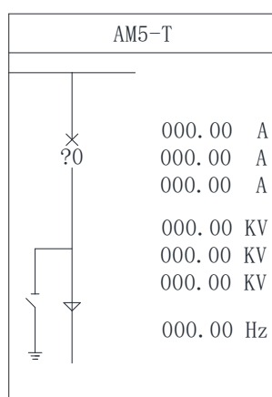
Fig 3.2 Mimic screen
